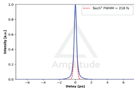
Pulse Duration
